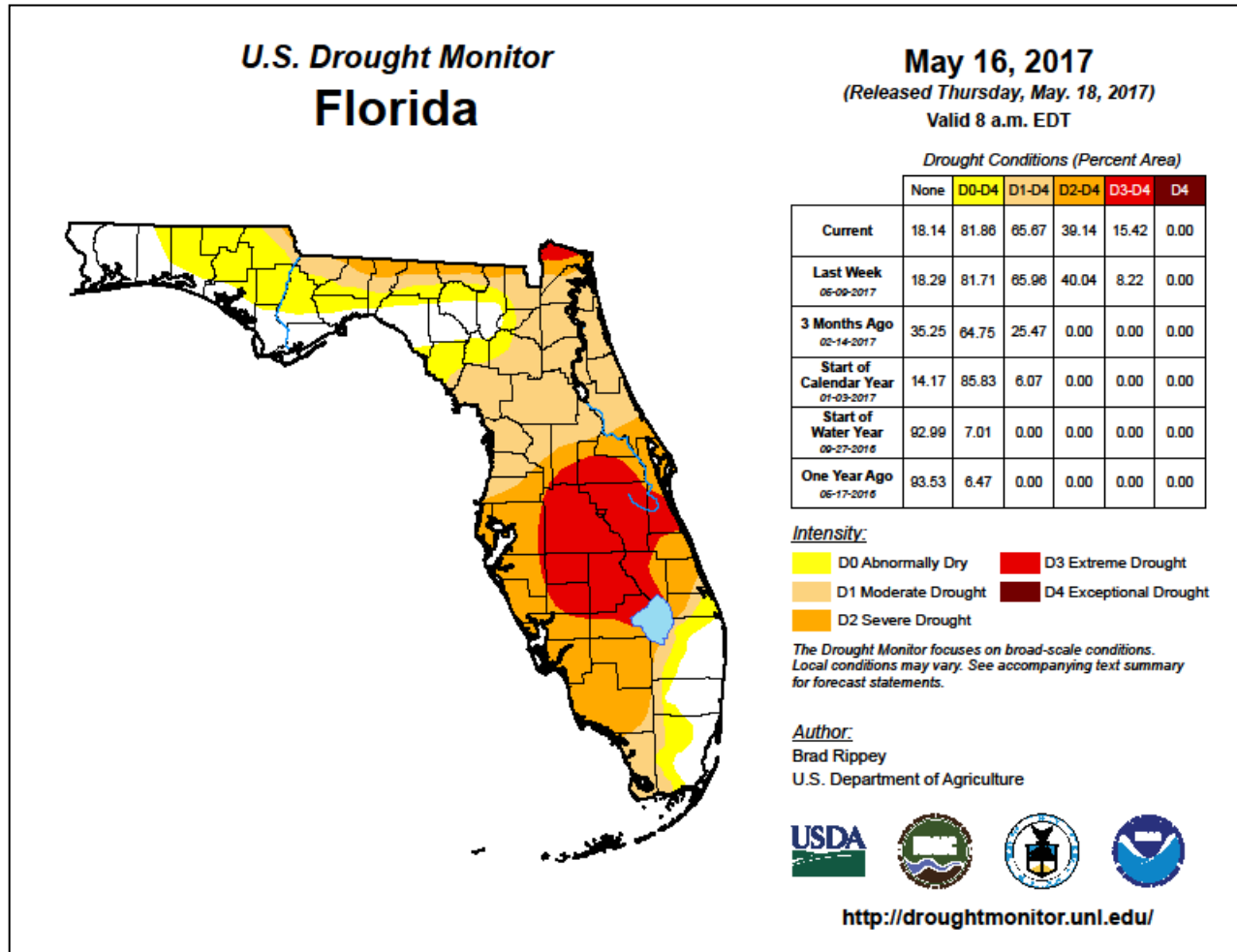
Figure 79: Florida U.S. Drought Monitor, May 2017 132
